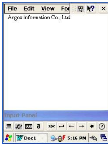
Figure 8-4 Transcriber
