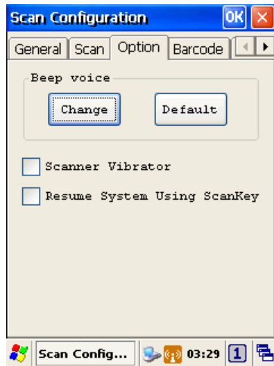
Figure 4-1-3 Scan Configuration
