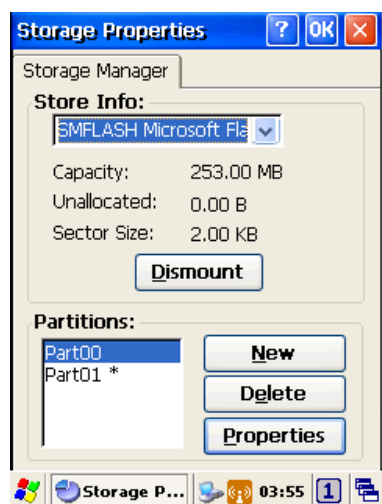
Figure 8-20 Storage Properties
