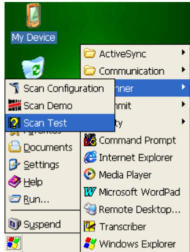
Figure 4-3-1 Scan Test
