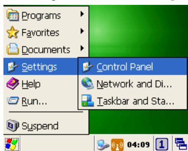
Figure 3-9 Backlight Setting
