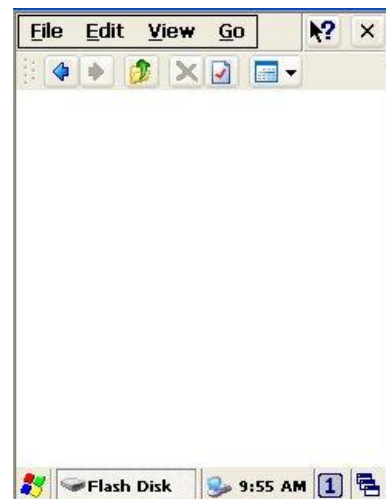
Figure 3-12-2 Flash Disk
