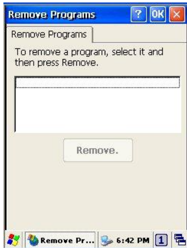
Figure 8-19 Remove Programs
