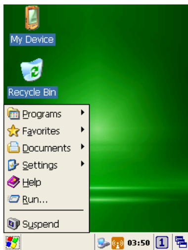
Figure 8-3 Start Icon
