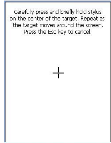
Figure 3-3 Calibration
