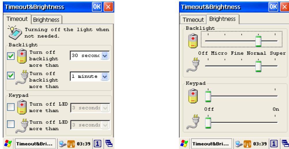
Figure 5-3 Timeout & Brightness
