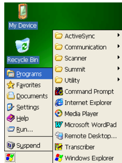
Figure 6-1 Programs Implemented
