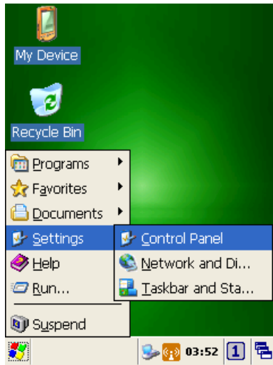
Figure 8-5 -1 Control Panel
