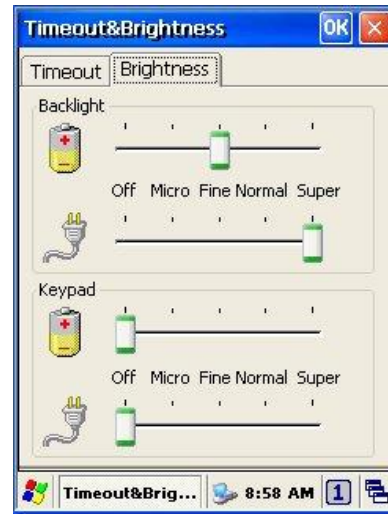
Figure 3-10 Timeout & Brightness
