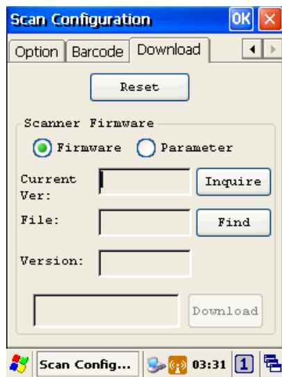
Figure 4-1 -4 Scan Configuration
