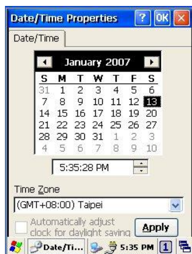
Figure 8-7 Date/Time
