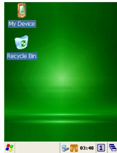
Figure 8-1 Main Window
