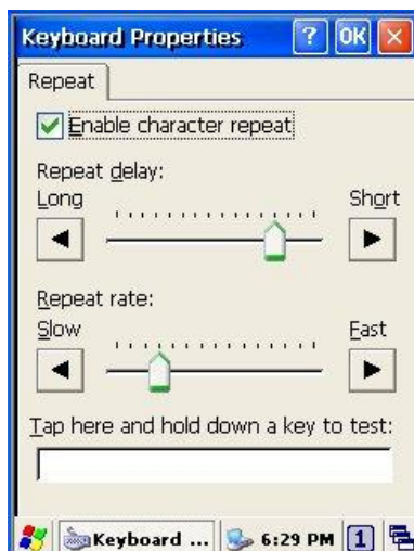
Figure 8-12 Keyboard Properties
