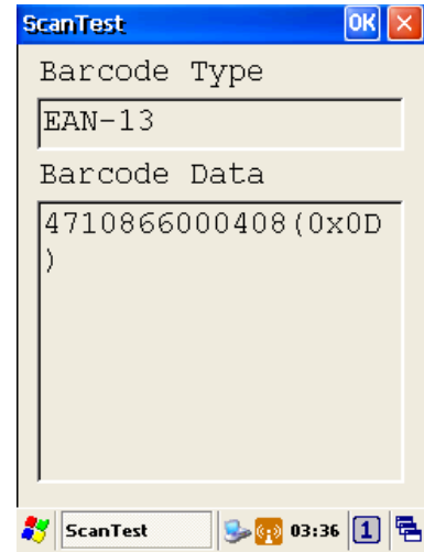
Figure 4-3-2 Scan Test
